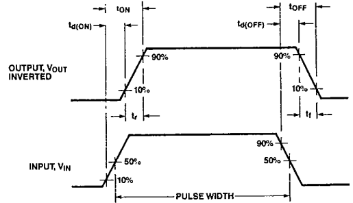
Figure 12 Switching Waveforms
