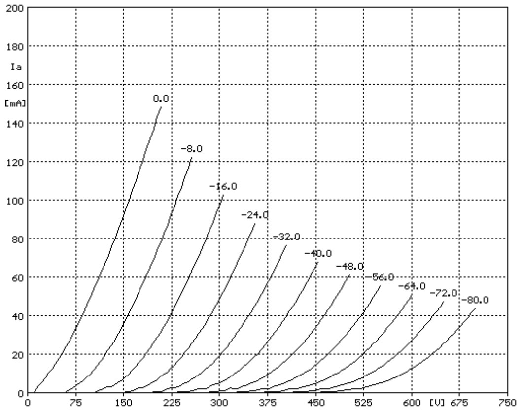
807 ultralinear mode connection
