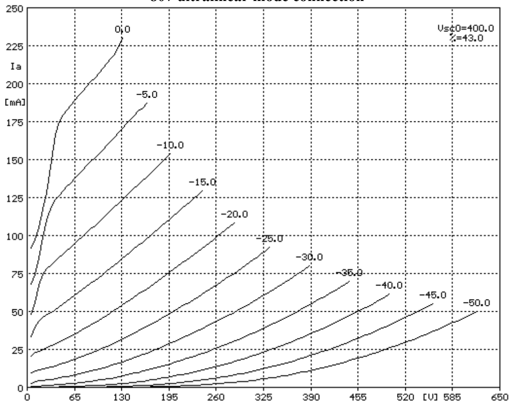
807 penthode mode connection
